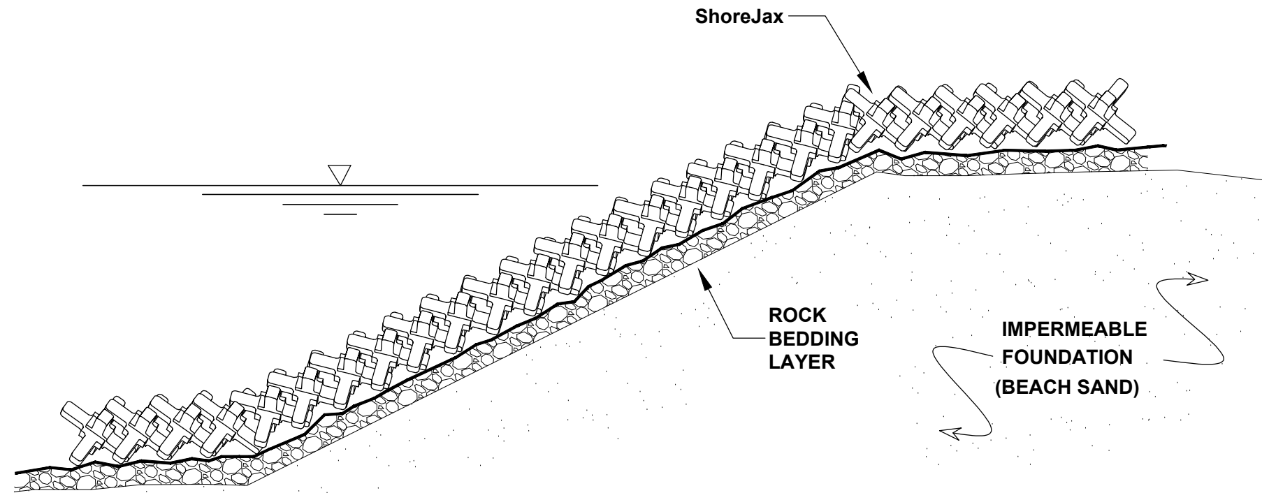
ShoreJax COASTAL PROTECTION NOT TO SCALE
