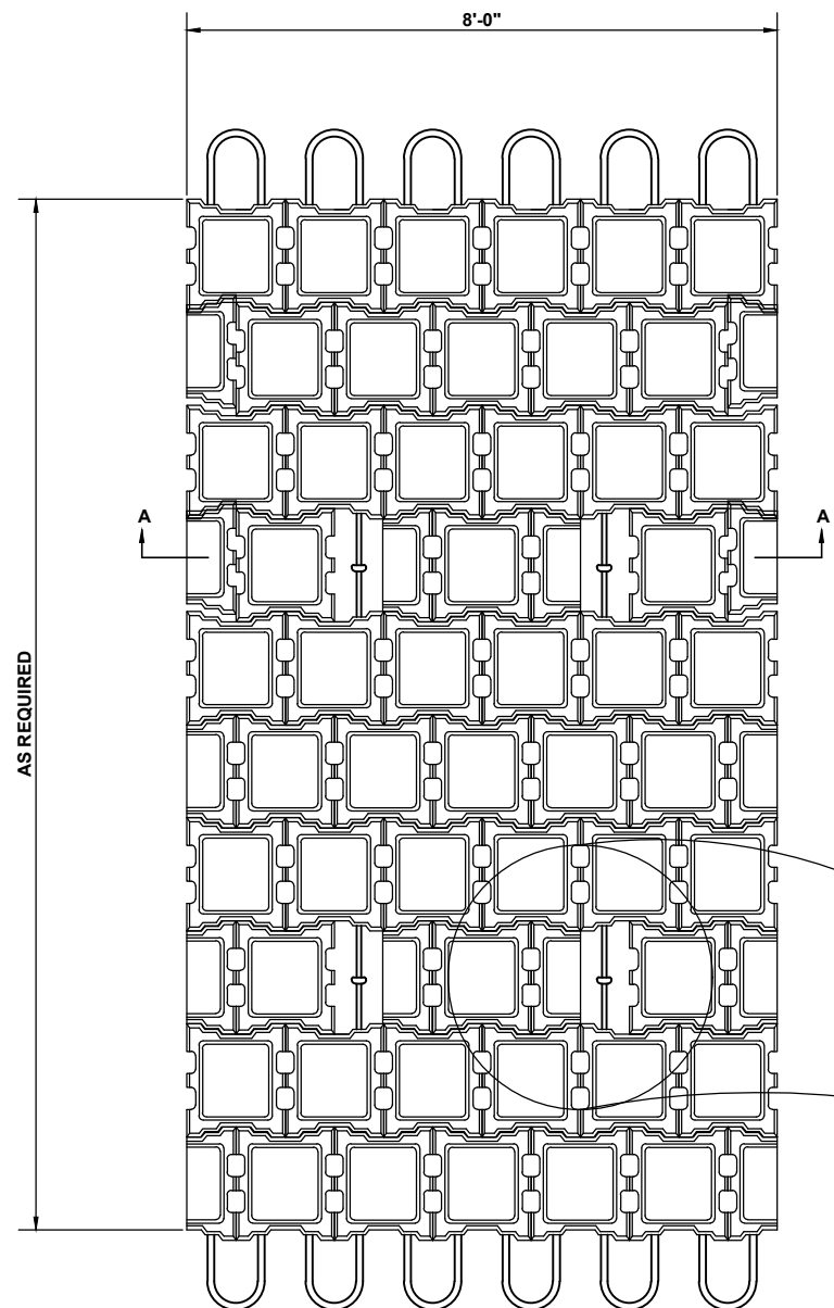
PLAN VIEW
