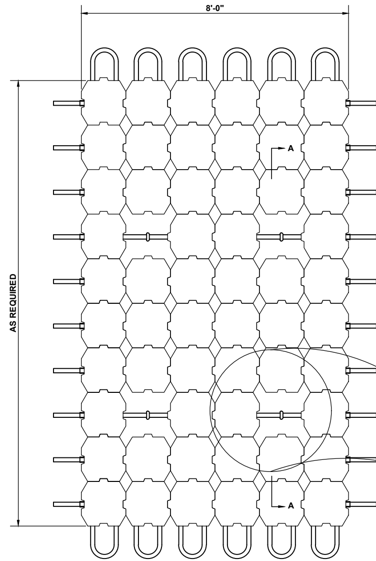
PLAN VIEW
