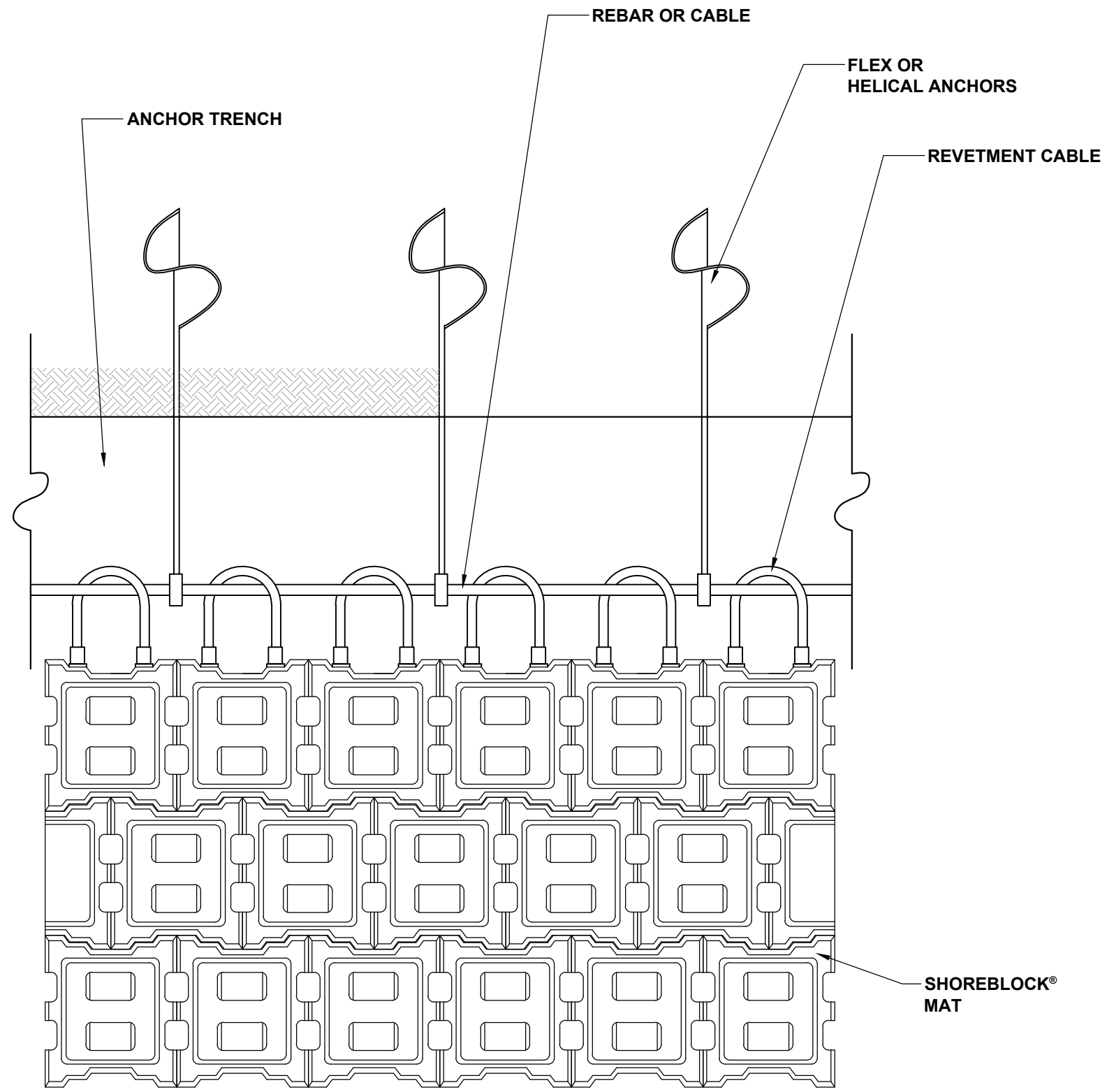
PLAN VIEW
