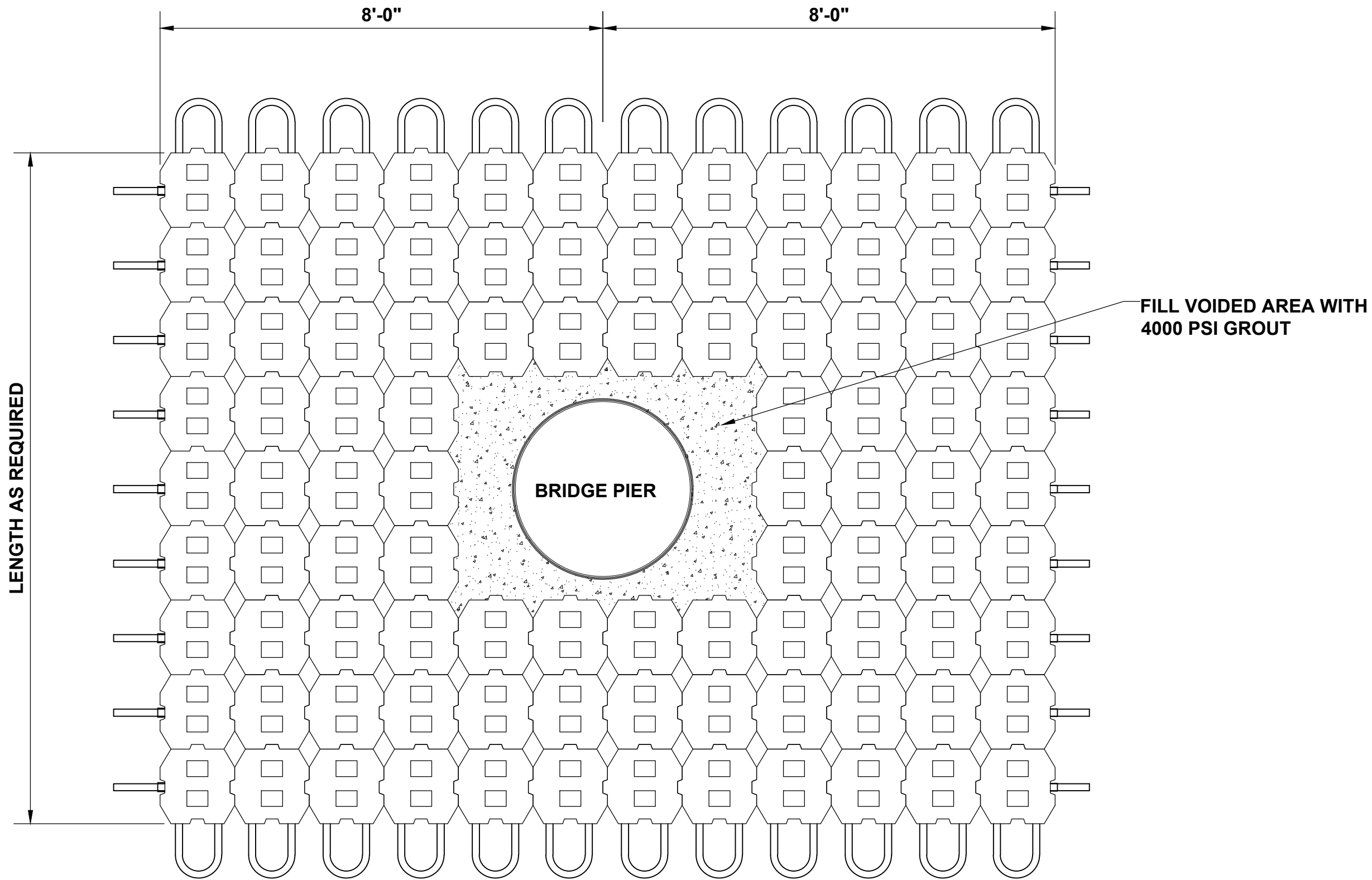
PLAN VIEW
