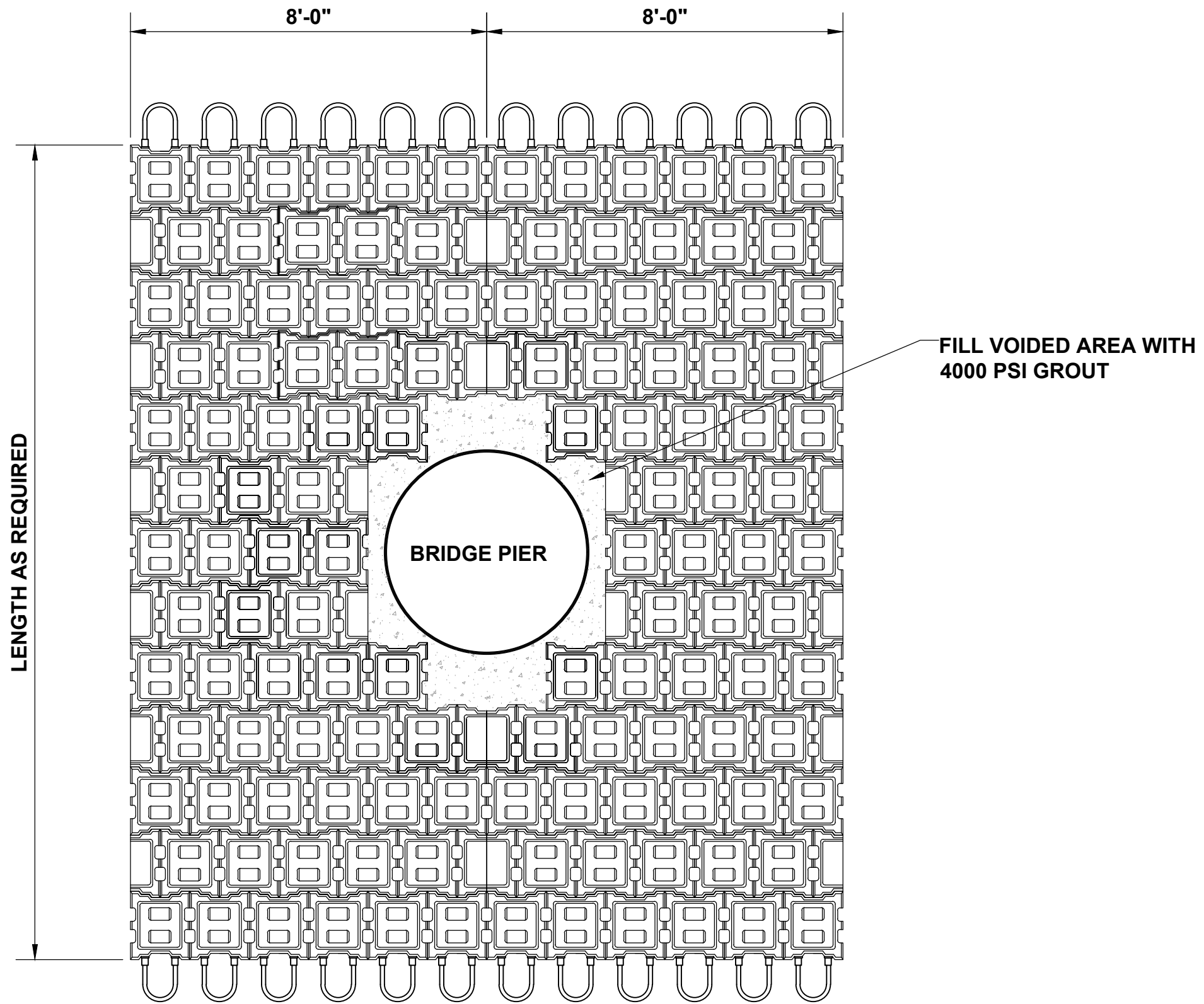
PLAN VIEW
