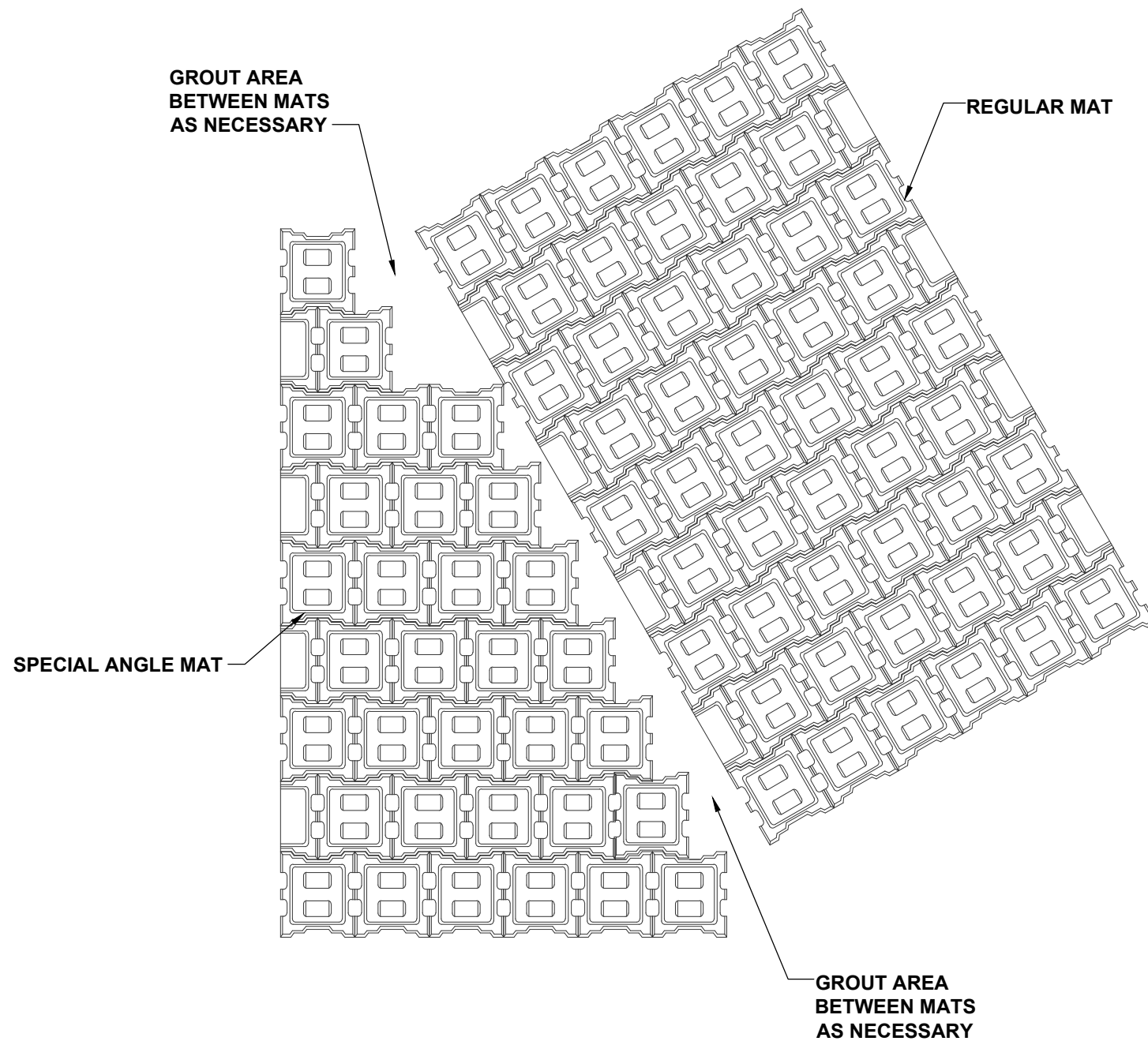
SPECIAL MATS (TYPICAL DETAIL)
