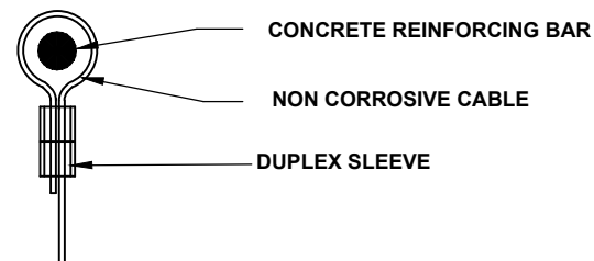
CONNECTION TYPE #2
