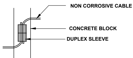
CONNECTION TYPE #1
