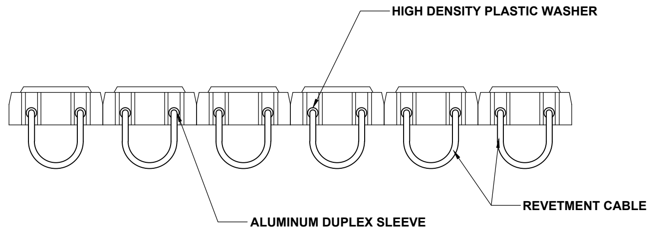
END VIEW
