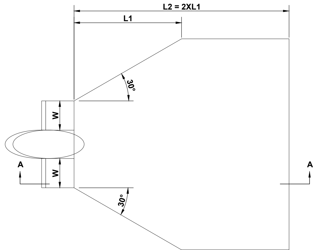
PLAN VIEW
