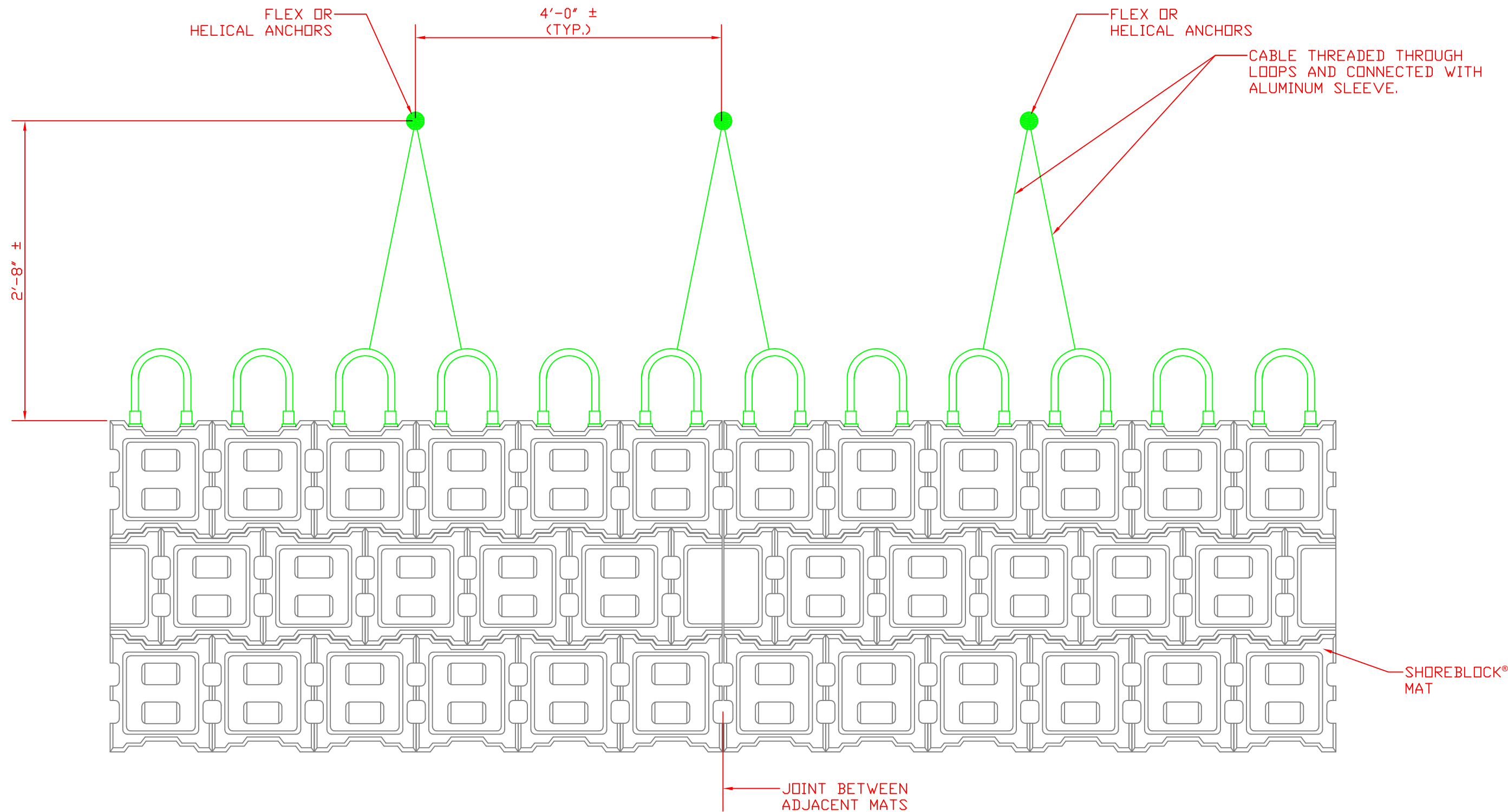
PLAN VIEW
