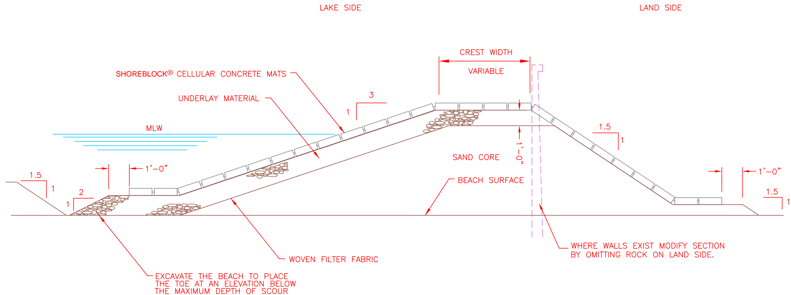
SECTION THRU DIKE
