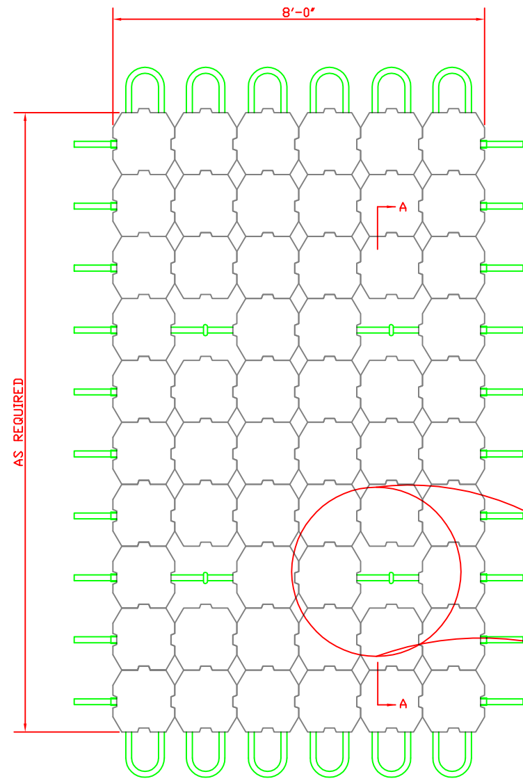
PLAN VIEW
