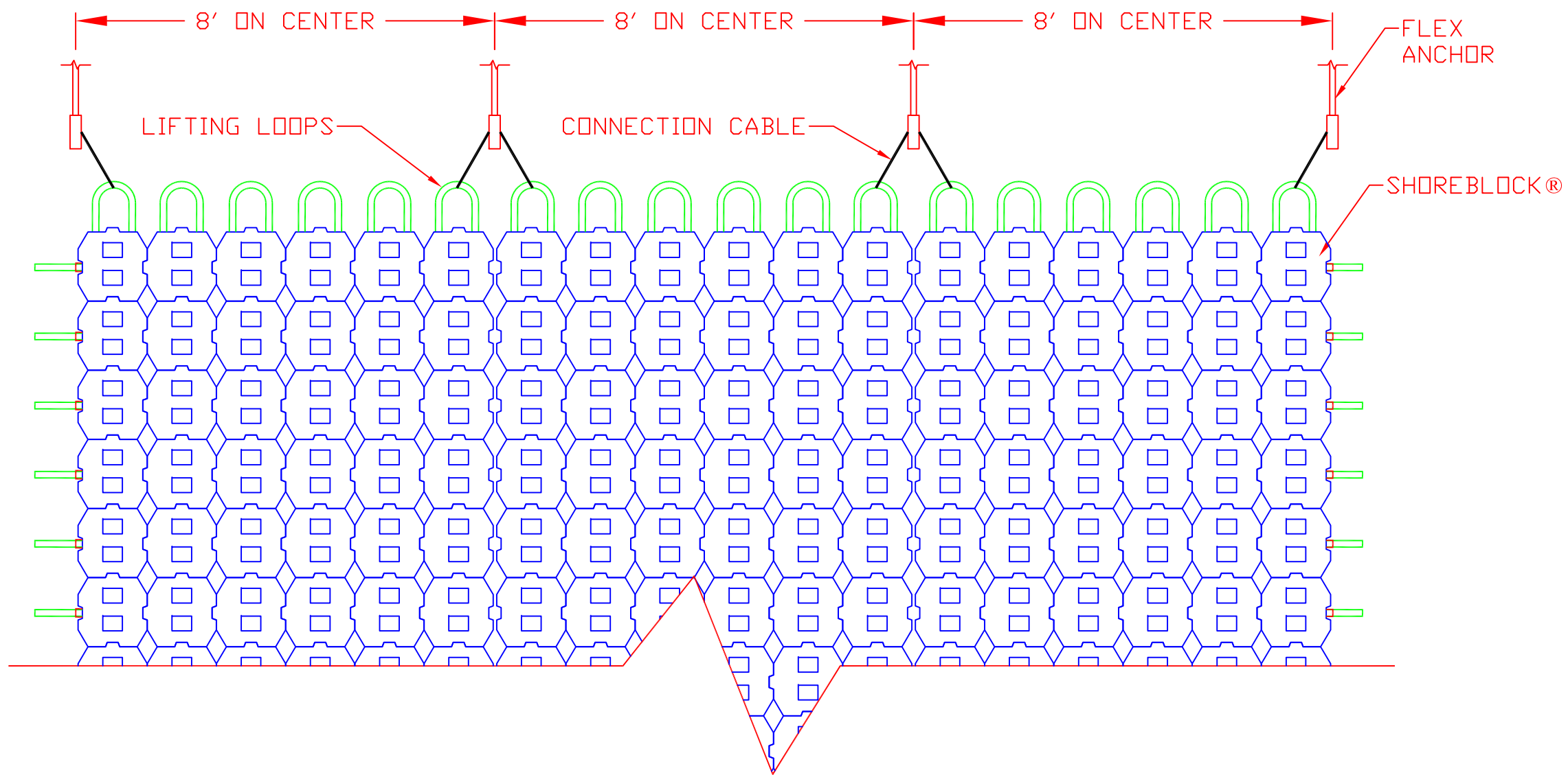
MECHANICAL FLEX ANCHORING PLACEMENT 8' ON CENTER
