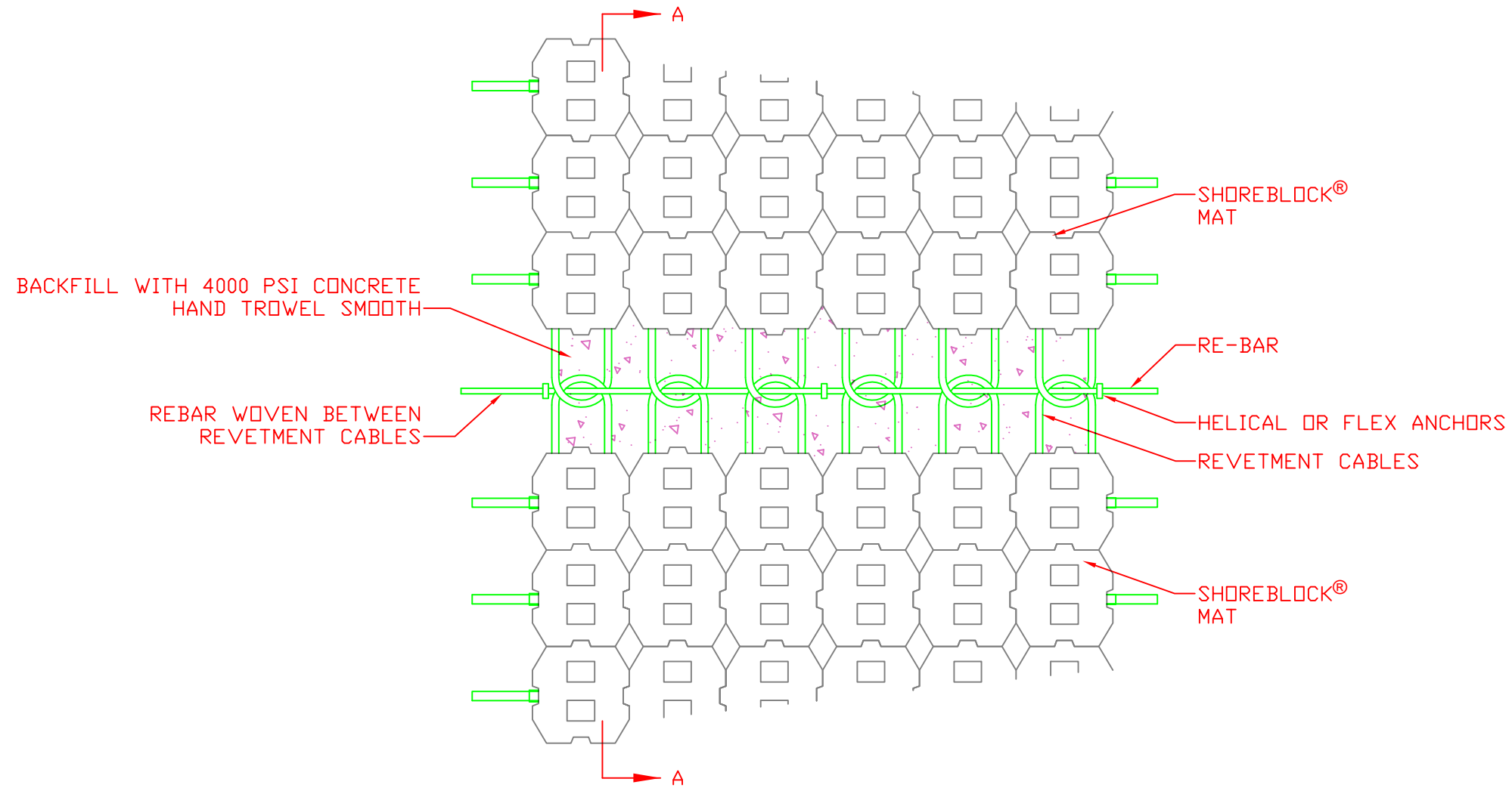
PLAN VIEW
