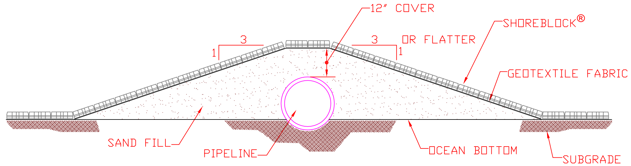
SECTION PIPELINE COVER
