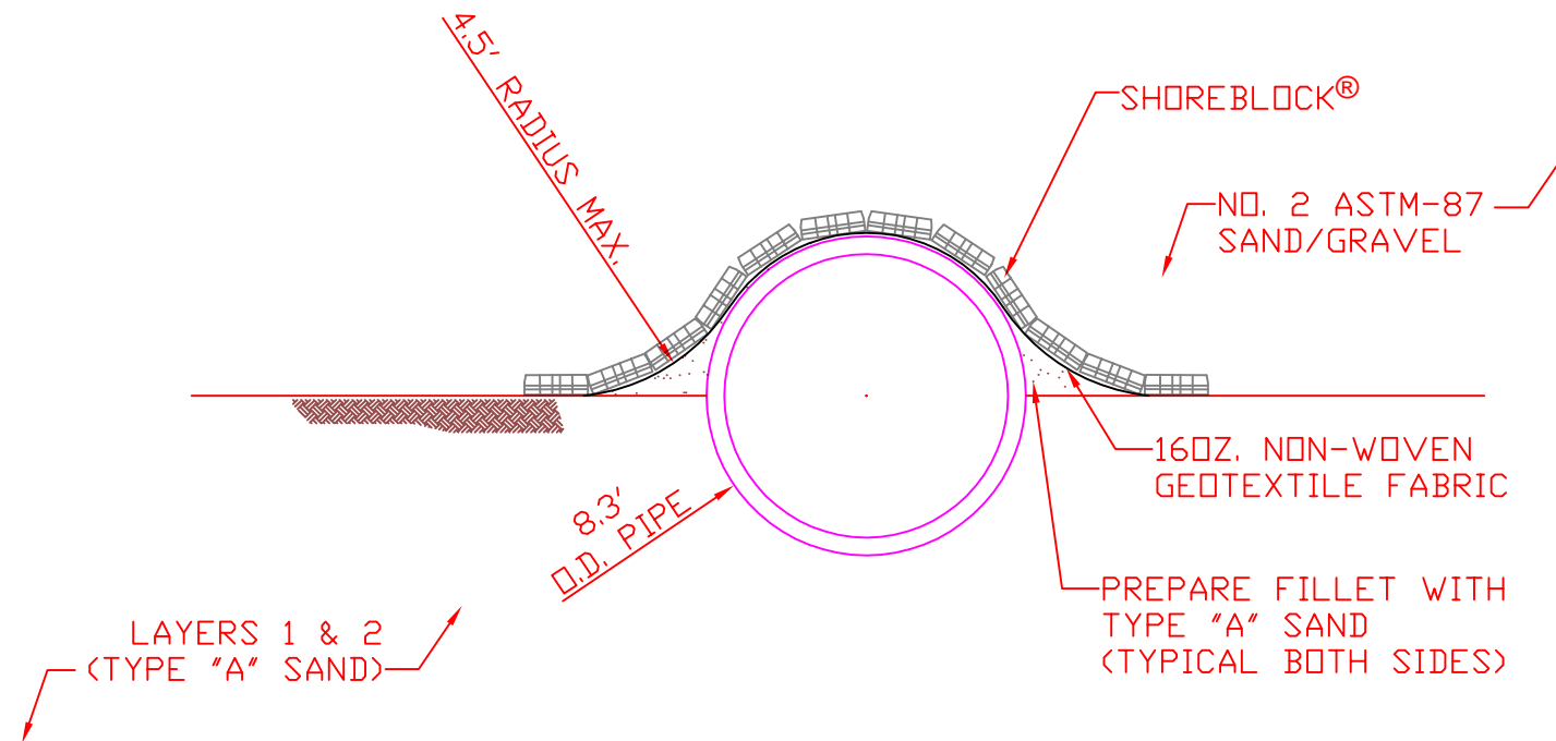
PIPELINE COVER SECTION
